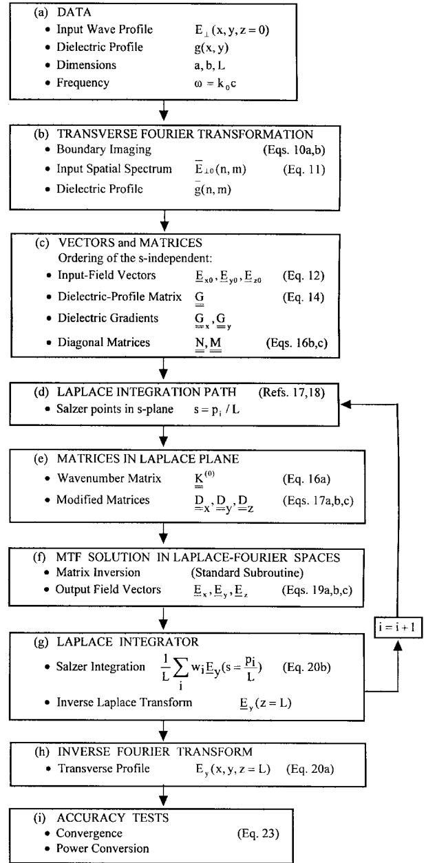
Fig. 3. A flowchart of the TMF computational algorithm.
