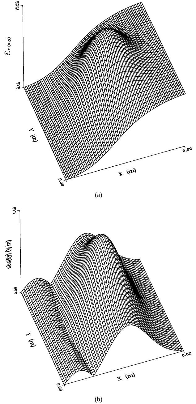
Fig. 10. A composition of a Gaussian profile dielectric rod and a slab with a diffused edge ( a = 2 cm, b = 1 cm, L = 17 cm, \lambda = 3.75 cm, and N = 9 ). (a) The dielectric profile \epsilon_r(x, y) . (b) The output field profile as a response to a half-sine input wave profile.
